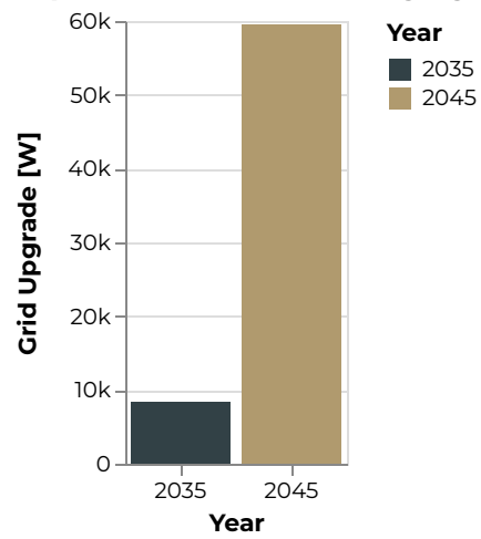
Figure 88: Toquerville Grid Upgrade [W]
