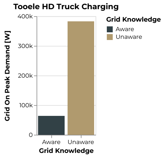
Figure 743: Tooele Grid On Peak Demand [W]
