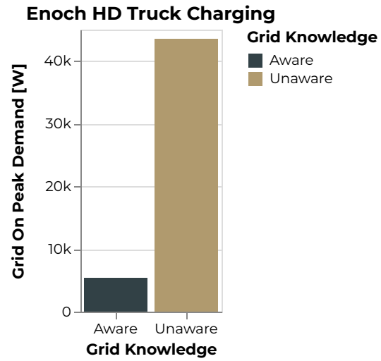
Figure 796: Enoch Grid On Peak Demand [W]
