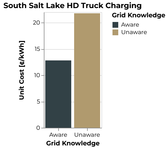
Figure 943: South Salt Lake Unit Cost [¢/kWh]
