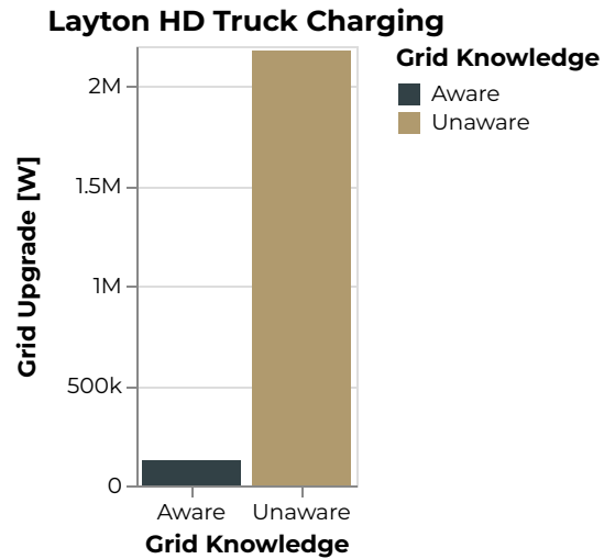
Figure 634: Layton Grid Upgrade [W]
