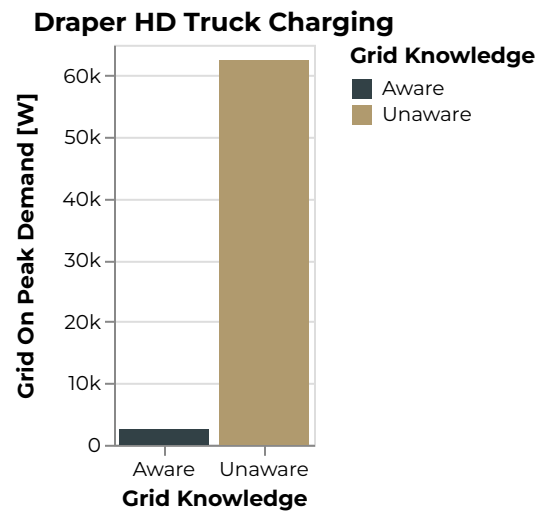
Figure 795: Draper Grid On Peak Demand [W]
