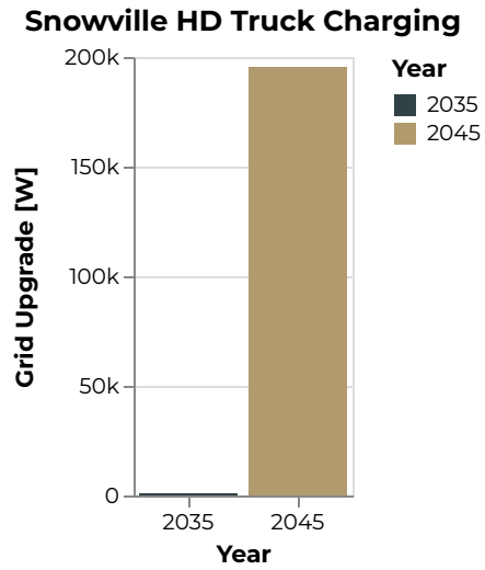
Figure 140: Snowville Grid Upgrade [W]
