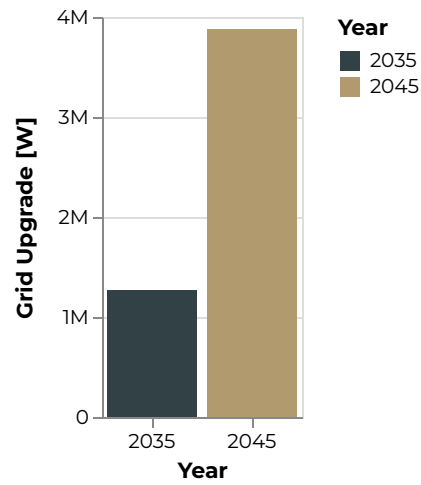
Figure 86: Bountiful Grid Upgrade [W]
