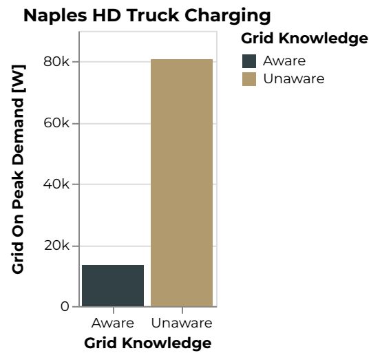
Figure 783: Naples Grid On Peak Demand [W]
