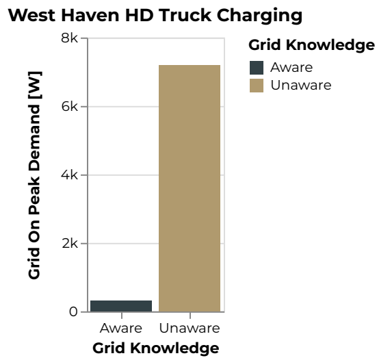
Figure 753: West Haven Grid On Peak Demand [W]
