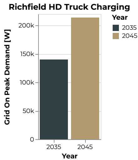
Figure 277: Richfield Grid On Peak Demand [W]
