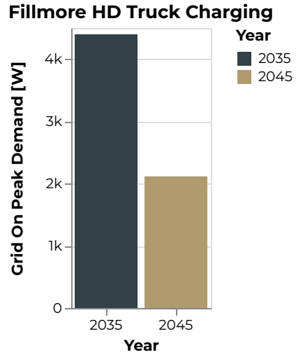
Figure 238: Fillmore Grid On Peak Demand [W]
