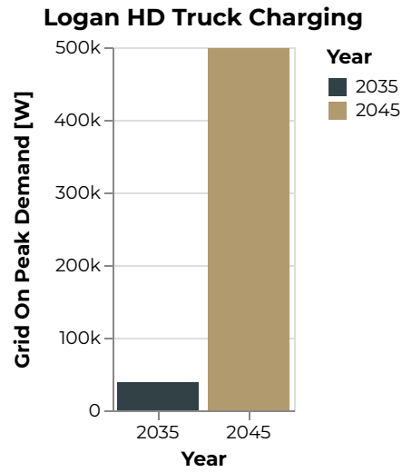
Figure 292: Logan Grid On Peak Demand [W]
