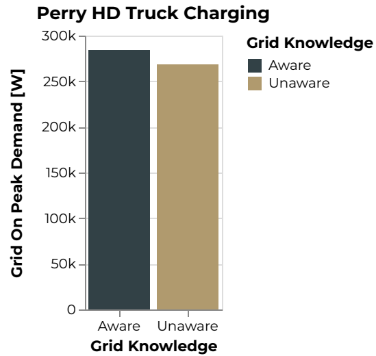
Figure 770: Perry Grid On Peak Demand [W]
