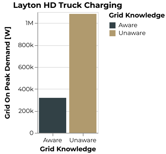
Figure 744: Layton Grid On Peak Demand [W]
