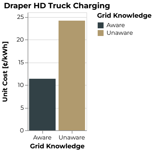
Figure 874: Draper Unit Cost [¢/kWh]
