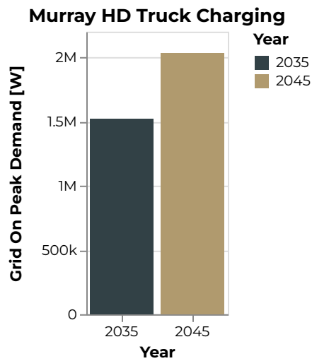
Figure 281: Murray Grid On Peak Demand [W]
