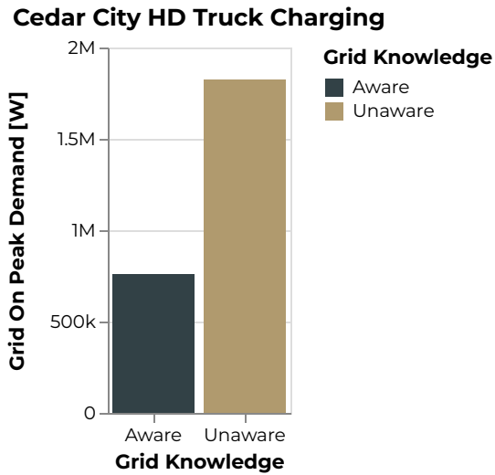
Figure 760: Cedar City Grid On Peak Demand [W]
