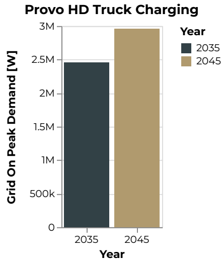
Figure 225: Provo Grid On Peak Demand [W]
