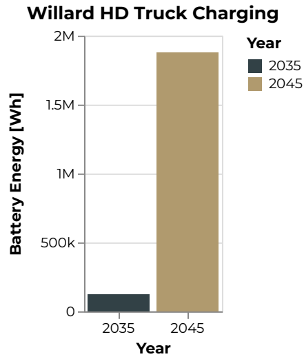
Figure 217: Willard Battery Energy [Wh]
