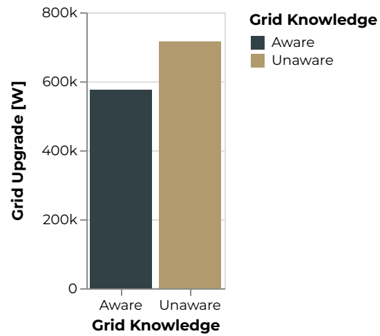
Figure 627: Green River Grid Upgrade [W]
