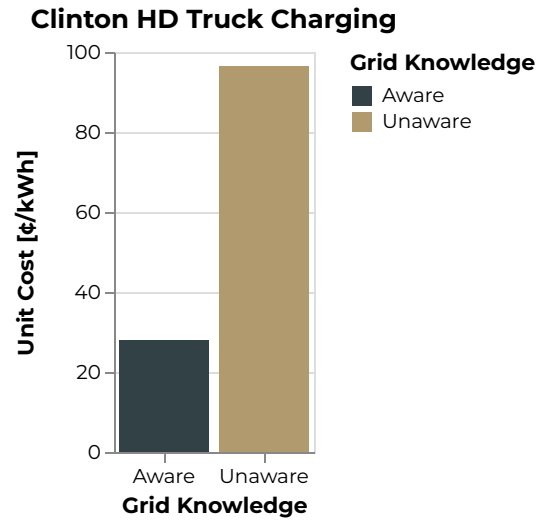
Figure 880: Clinton Unit Cost [¢/kWh]
