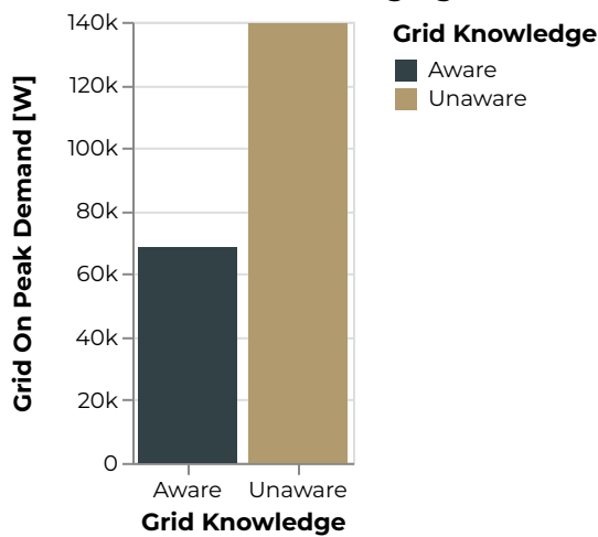
Figure 773: Riverton Grid On Peak Demand [W]
