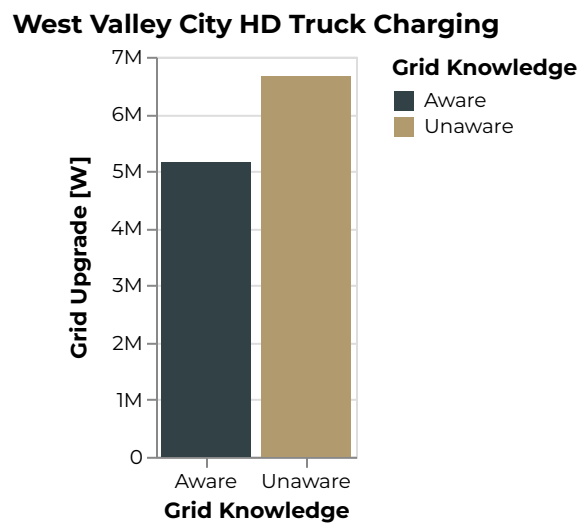
Figure 587: West Valley City Grid Upgrade [W]
