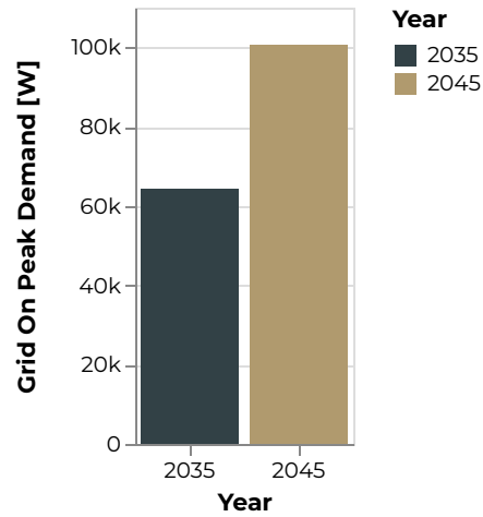
Figure 228: Saratoga Springs Grid On Peak Demand [W]
