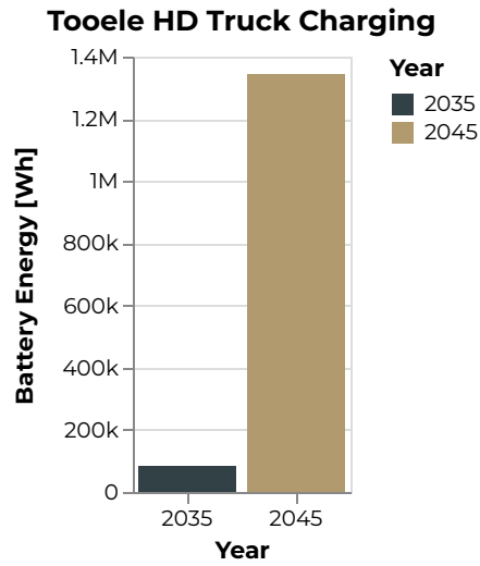
Figure 210: Tooele Battery Energy [Wh]
