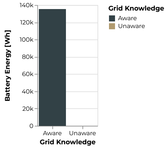
Figure 719: Millville Battery Energy [Wh]
