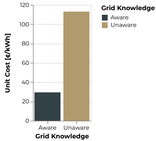
Figure 881: Orem Unit Cost [¢/kWh]
