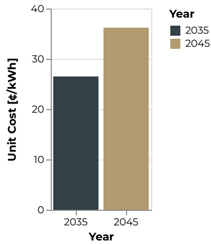
Figure 392: Willard Unit Cost [¢/kWh]
