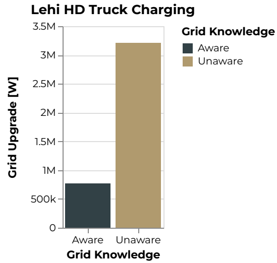
Figure 612: Lehi Grid Upgrade [W]
