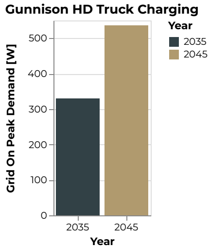
Figure 280: Gunnison Grid On Peak Demand [W]
