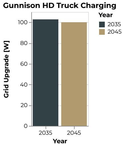
Figure 84: Gunnison Grid Upgrade [W]
