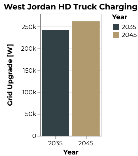
Figure 121: West Jordan Grid Upgrade [W]
