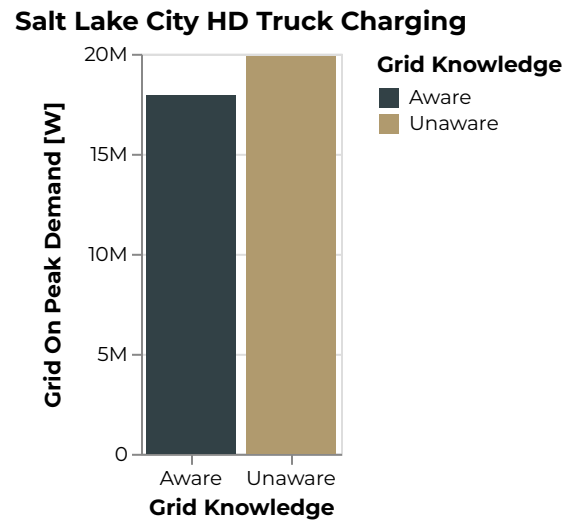
Figure 793: Salt Lake City Grid On Peak Demand [W]
