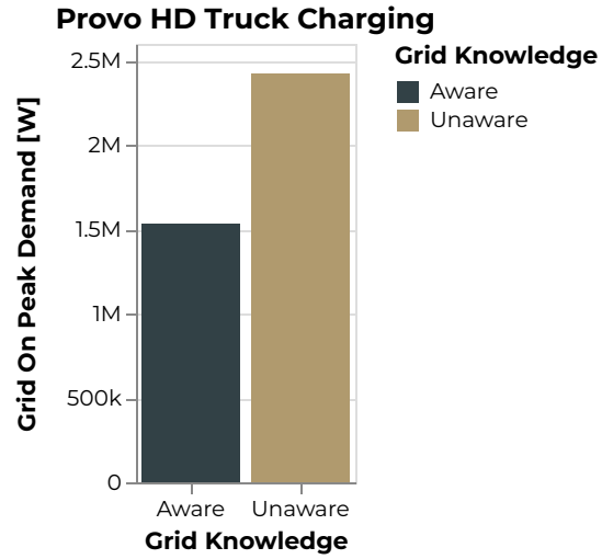
Figure 778: Provo Grid On Peak Demand [W]
