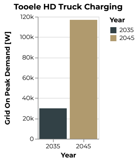
Figure 289: Tooele Grid On Peak Demand [W]
