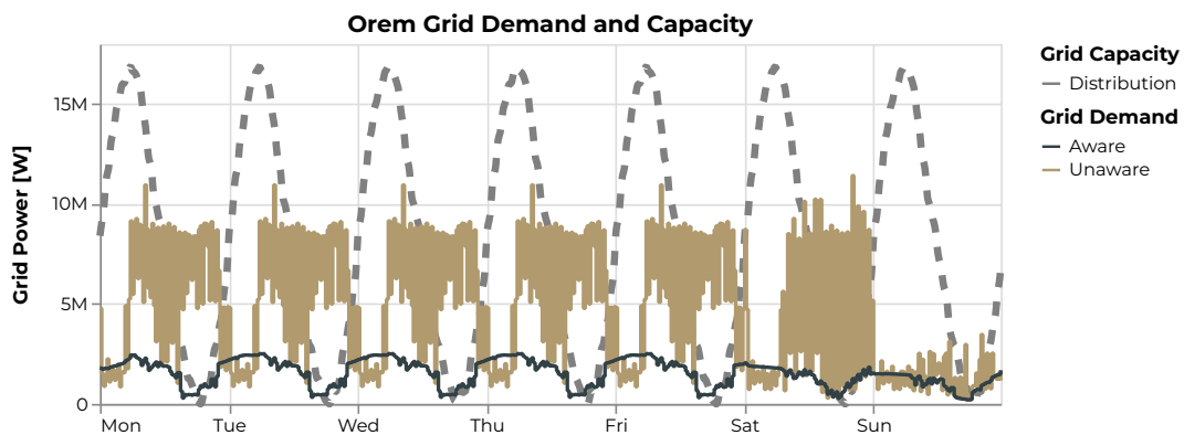
Figure 6: Orem grid demand compared with capacity for grid-aware and grid-unaware cases.
