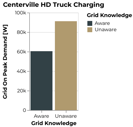
Figure 775: Centerville Grid On Peak Demand [W]
