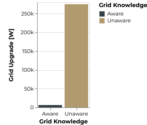
Figure 622: South Salt Lake Grid Upgrade [W]
