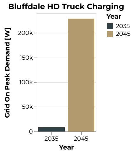
Figure 253: Bluffdale Grid On Peak Demand [W]
