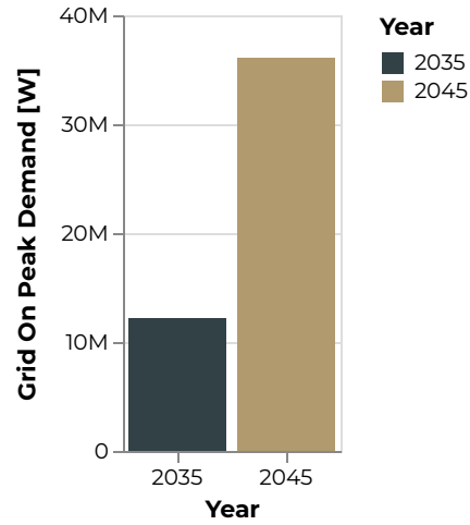
Figure 294: Salt Lake City Grid On Peak Demand [W]
