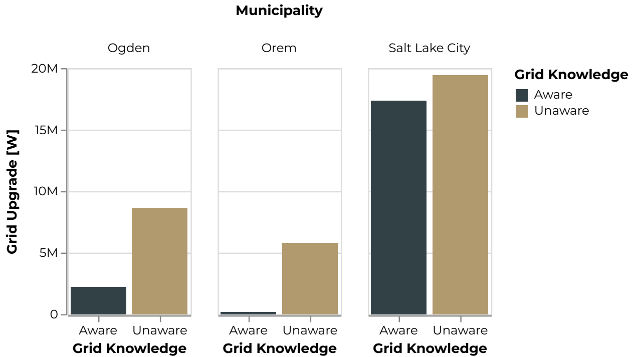
Figure 4: Required grid upgrades for selected municipalities by grid-awareness case.
