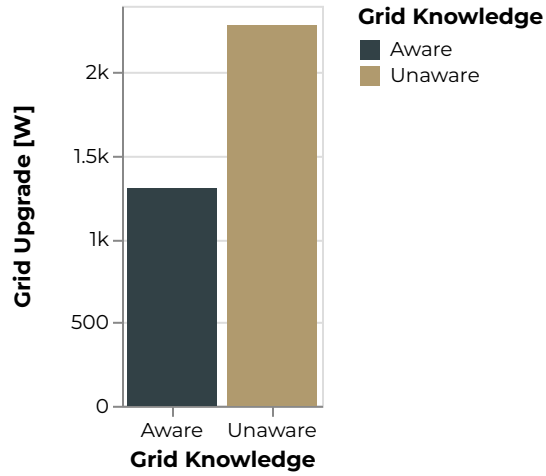
Figure 645: American Fork Grid Upgrade [W]
