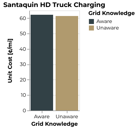
Figure 972: Santaquin Unit Cost [¢/mi]
