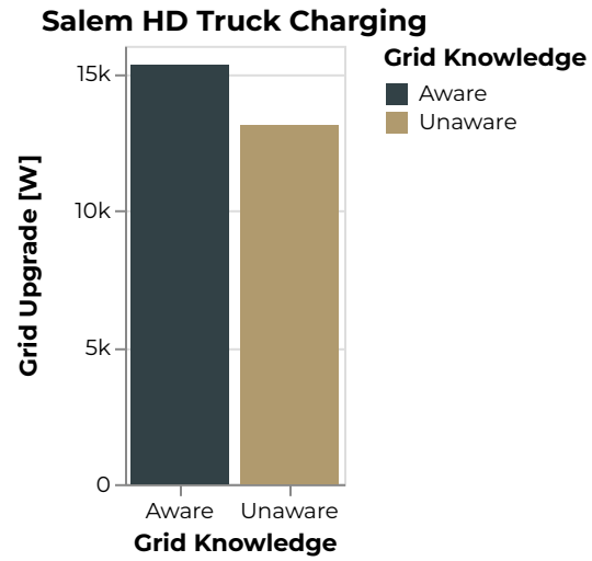
Figure 629: Salem Grid Upgrade [W]
