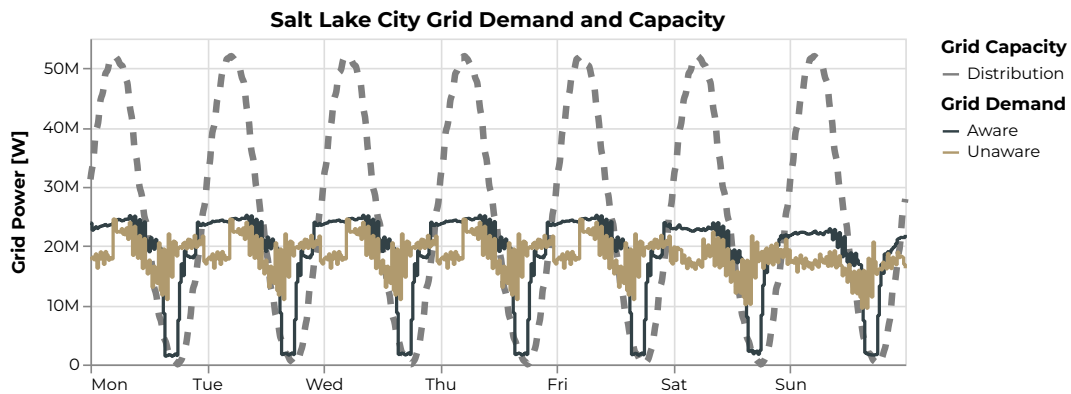
Figure 5: Salt Lake City grid demand compared with capacity for grid-aware and grid-unaware cases.
