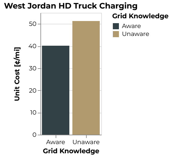
Figure 1009: West Jordan Unit Cost [¢/mi]
