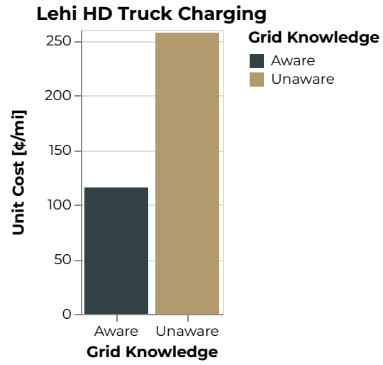
Figure 970: Lehi Unit Cost [¢/mi]
