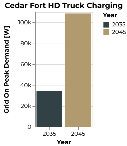
Figure 290: Cedar Fort Grid On Peak Demand [W]
