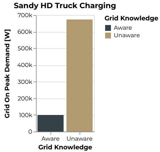
Figure 730: Sandy Grid On Peak Demand [W]
