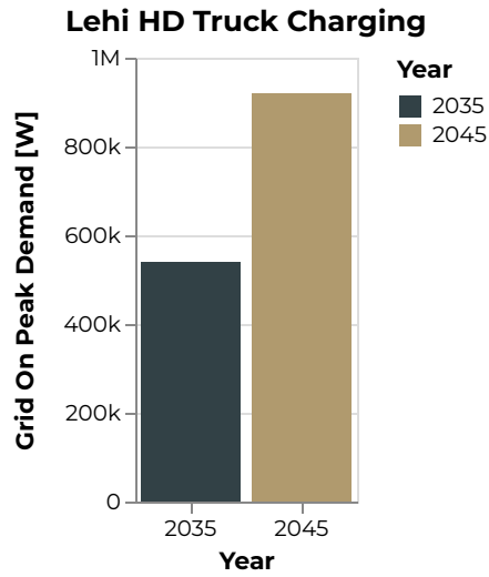
Figure 224: Lehi Grid On Peak Demand [W]
