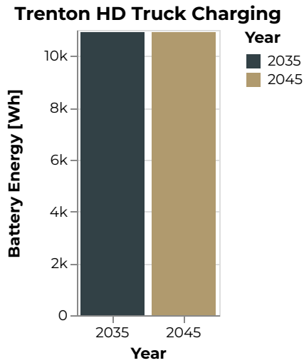
Figure 188: Trenton Battery Energy [Wh]
