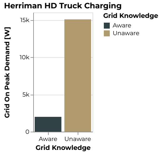
Figure 771: Herriman Grid On Peak Demand [W]
