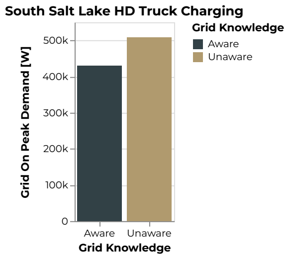
Figure 759: South Salt Lake Grid On Peak Demand [W]
