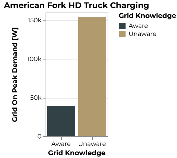
Figure 728: American Fork Grid On Peak Demand [W]
