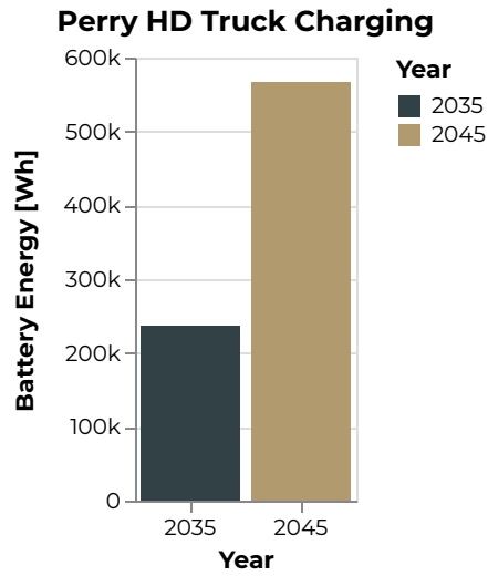
Figure 172: Perry Battery Energy [Wh]
