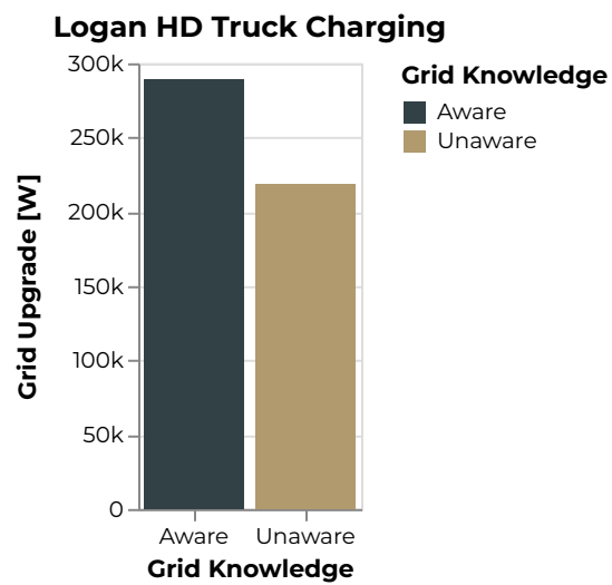
Figure 635: Logan Grid Upgrade [W]
