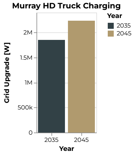
Figure 95: Murray Grid Upgrade [W]
