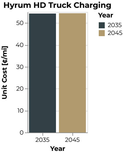
Figure 481: Hyrum Unit Cost [¢/mi]
