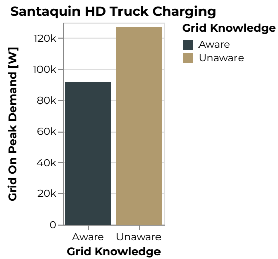
Figure 749: Santaquin Grid On Peak Demand [W]
