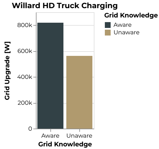
Figure 630: Willard Grid Upgrade [W]
