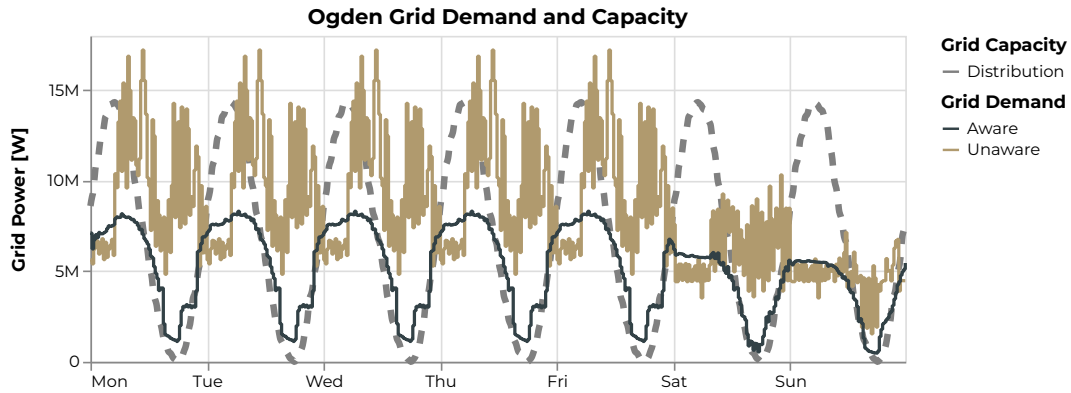
Figure 7: Ogden grid demand compared with capacity for grid-aware and grid-unaware cases.
