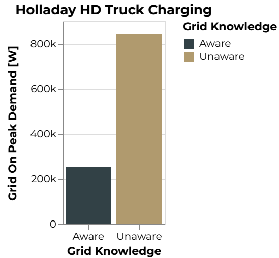
Figure 752: Holladay Grid On Peak Demand [W]
