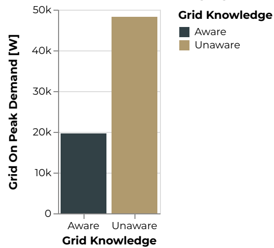
Figure 762: Pleasant Grove Grid On Peak Demand [W]
