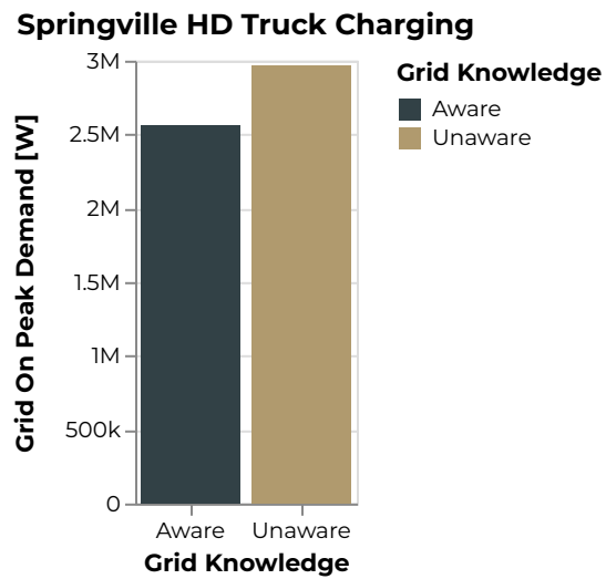
Figure 767: Springville Grid On Peak Demand [W]
