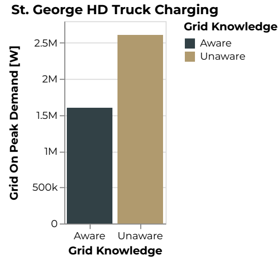
Figure 785: St. George Grid On Peak Demand [W]
