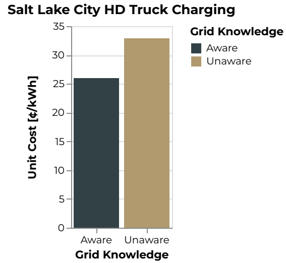
Figure 938: Salt Lake City Unit Cost [¢/kWh]
