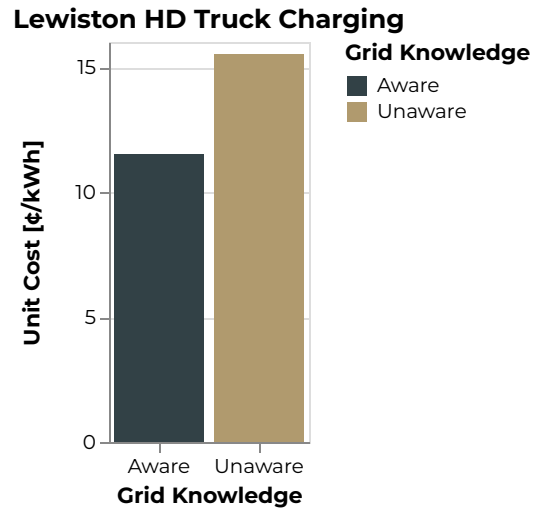
Figure 918: Lewiston Unit Cost [¢/kWh]
