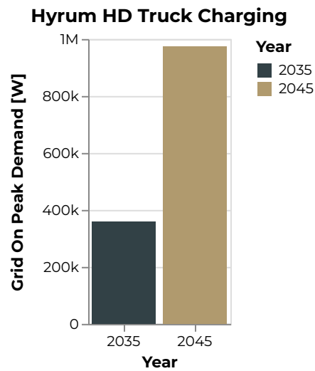
Figure 285: Hyrum Grid On Peak Demand [W]
