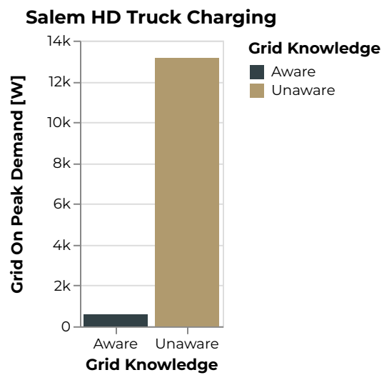
Figure 733: Salem Grid On Peak Demand [W]
