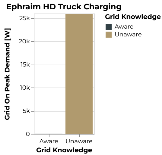
Figure 757: Ephraim Grid On Peak Demand [W]
