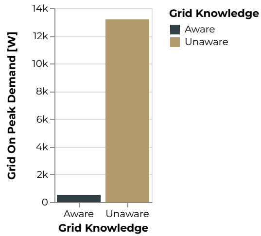
Figure 768: Toquerville Grid On Peak Demand [W]
