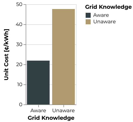
Figure 893: Ogden Unit Cost [¢/kWh]
