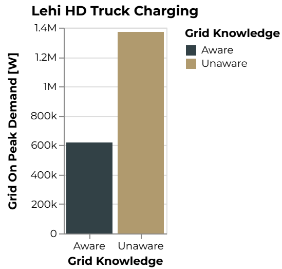
Figure 761: Lehi Grid On Peak Demand [W]
