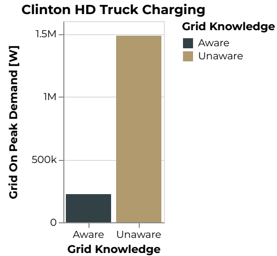
Figure 734: Clinton Grid On Peak Demand [W]
