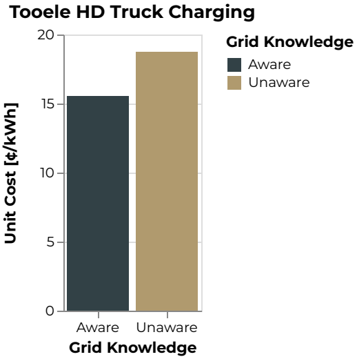
Figure 928: Tooele Unit Cost [¢/kWh]
