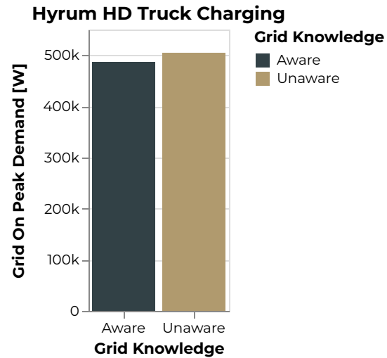
Figure 754: Hyrum Grid On Peak Demand [W]
