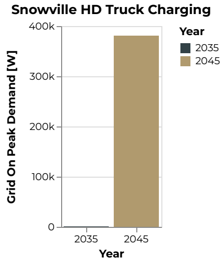
Figure 256: Snowville Grid On Peak Demand [W]
