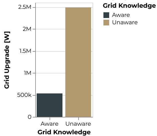
Figure 638: South Jordan Grid Upgrade [W]
